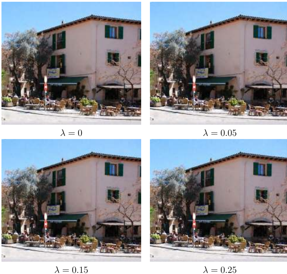
Figure 6: \sigma = 10
