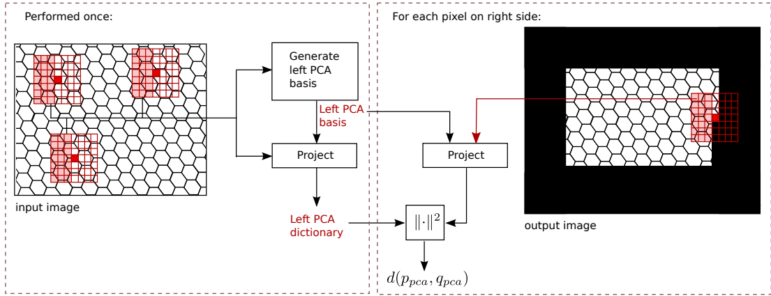
Figure 2: The left PCA basis is created from all the left-halves of patches in the sample image. Then the left dictionary is created, containing the projections of all the left-halves of patches in the sample image onto the left PCA basis. To fill a pixel for which the left half has already been synthesized, the known half of the corresponding patch is projected onto the left PCA basis and the distance to all elements of the left dictionary are computed. The algorithm continues as for the classical case. The same procedure is performed for the right, top and bottom side cases.
