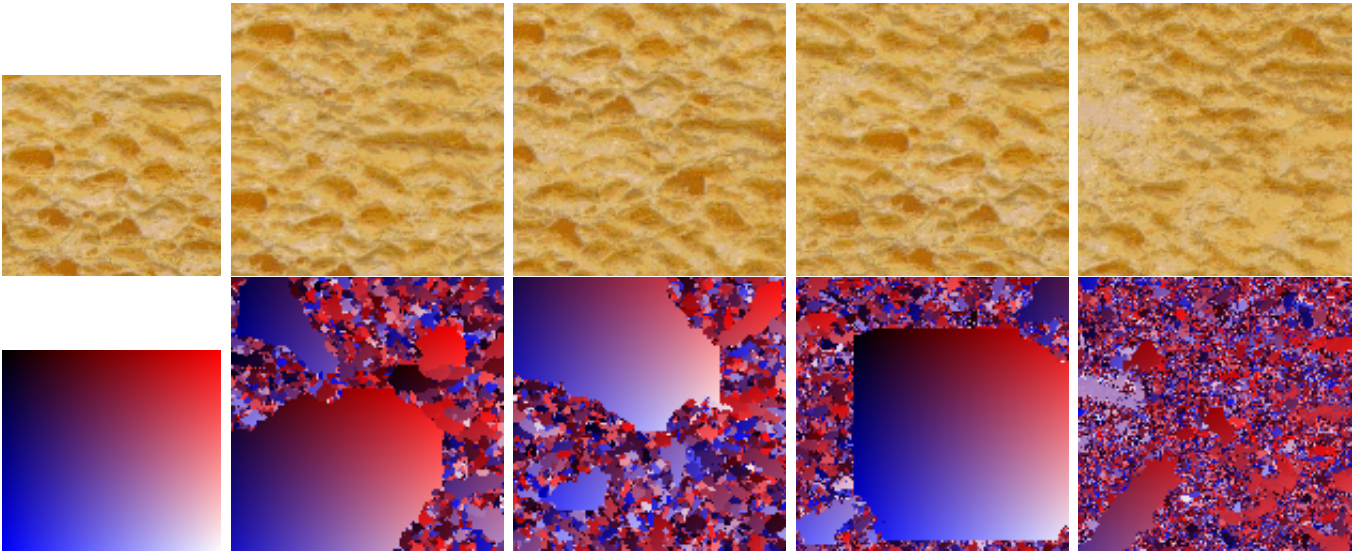
Figure 8: Tolerance parameter variation. First row (from left to right): sample image, results obtained with \varepsilon taking values 0.05, 0.1, 0.3, and 0.5. The patch size is set to 9. Second row: Corresponding synthesis maps. The innovation capacity of the method increases with \varepsilon , as can be verified in the increasingly noisy aspect of the synthesis maps. Results are good for small \varepsilon values, but are essentially made of small regions from the exemplar that are stitched together. Results are very noisy for large \varepsilon .
