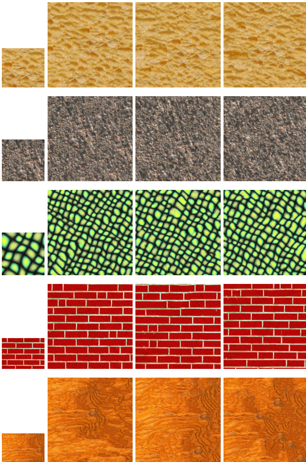
Figure 12: Reproducibility of results. Each row presents synthesis results on a texture from [8]. From left to right: sample image, result by Efron and Leung taken from [8], result obtained using our implementation of the method, result obtained using our accelerated version. Each time, all three results are visually very similar.
