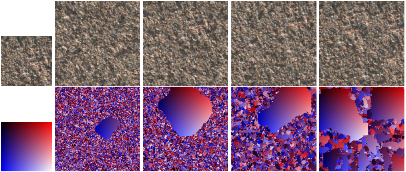
Figure 5: Patch size variation. First row (from left to right): sample image, results obtained with patch sizes 3, 5, 9, and 17. Second row: Corresponding synthesis maps. Good results are obtained in all cases. The innovation capacity decreases with increasing n , as can be verified in the decreasingly noisy aspect of the synthesis maps.
