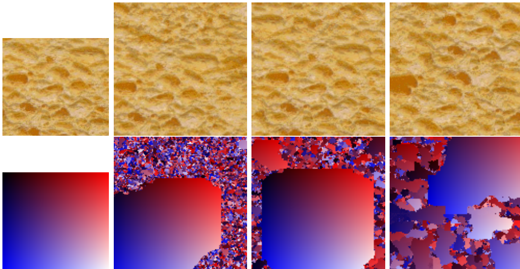
Figure 6: Patch size variation. First row (from left to right): sample image, results obtained with patch sizes 5, 9, and 17. Second row: Corresponding synthesis maps. Unlike the previous example (figure 5), the regions of the output images which are not verbatim copied do not faithfully represent the sample image.
