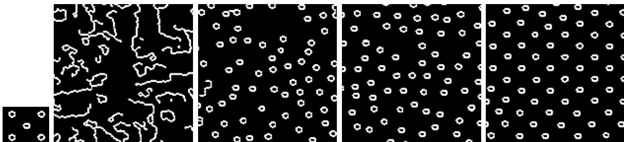
Figure 4: Texture scale. From left to right: sample image, results obtained with patch widths 5, 11, 15, and 23. The original image is from the Efros–Leung paper [8] and results are obtained with our implementation. A patch size of 5 is too small to recreate the circles of diameter 10. A patch size of 11 can represent the circles but not their spatial pattern. Increasing the patch size to 23 gives a correct result.
