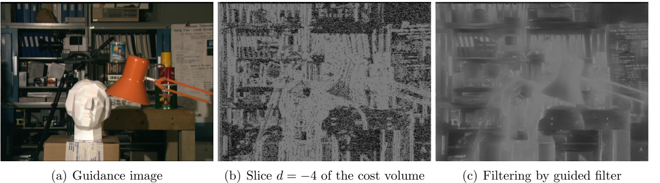
Figure 4: Filtering by guided filter of a slice of the cost volume for the Tsukuba pair ( \tau_1 = 7 , \tau_2 = 2 , \alpha = 0.9 , \varepsilon = 10^{-4} , r_{\text{GF}} = 9 ).
