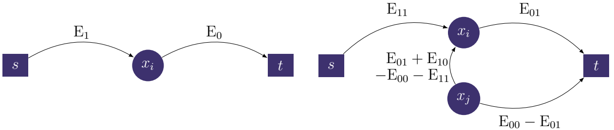
(a) Representation of a unary function (go to Figure 17 in Appendix B to see the cuts). (b) Representation of a pairwise function (go to Figure 18 in Appendix B to see the cuts).
