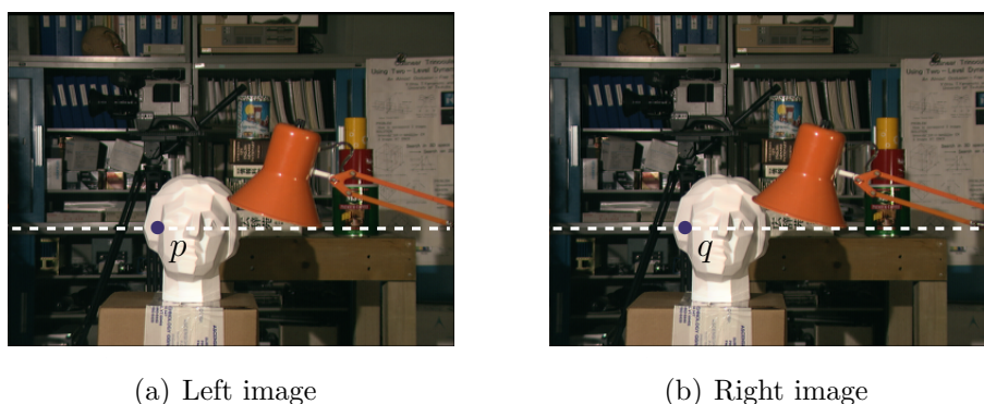
Figure 2: Point p corresponds to q . The white dashed lines are the corresponding epipolar lines.
