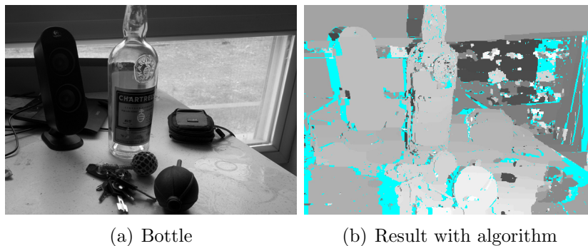
Figure 10: Results of the algorithm on the Bottle pair.
