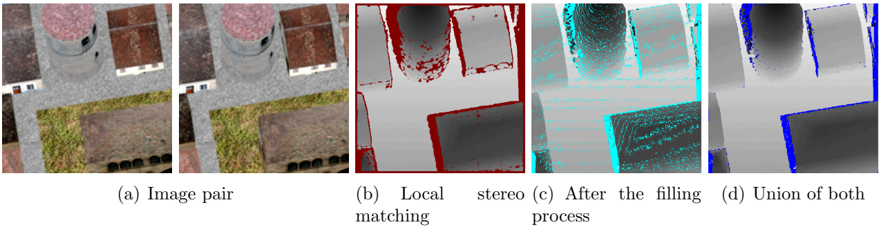
Figure 12: The initial disparity map was obtained by a block-matching method where the red pixels have been rejected by several filters (left-right/right-left consistency check, self similarity and flat patch detection). After the filling process by graph cuts, “occluded” pixels were marked in cyan. After replacing the “occluded” pixels that had an initial disparity, we get a denser map, with final rejected pixels in blue.
