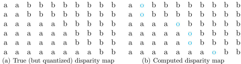
Figure 9: Combined effect of quantification and uniqueness constraint on computed disparity of a slanted roughly uniform surface. We assume a = b + 1 and o is the occlusion label.
