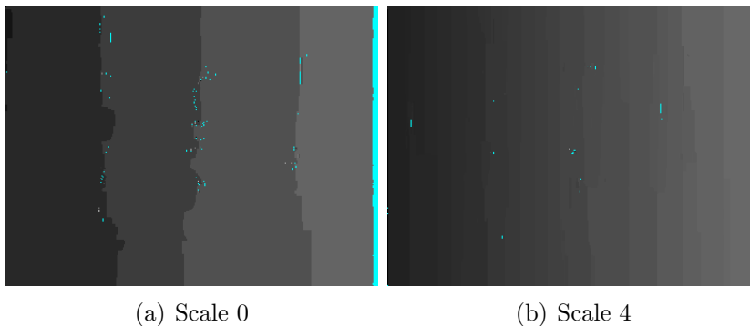
Figure 14: Synthetic disparity ramp applied to left Tsukuba image: d(p) = ap_x + b , with a = 0.01 and b = 1.5 . Left: pixel accurate recovered disparity map. Right: 1/16^{\text{th}} -pixel accurate recovered disparity map through multiscale refinement. For such a disparity map subpixel precision is needed to avoid quantification effects.
