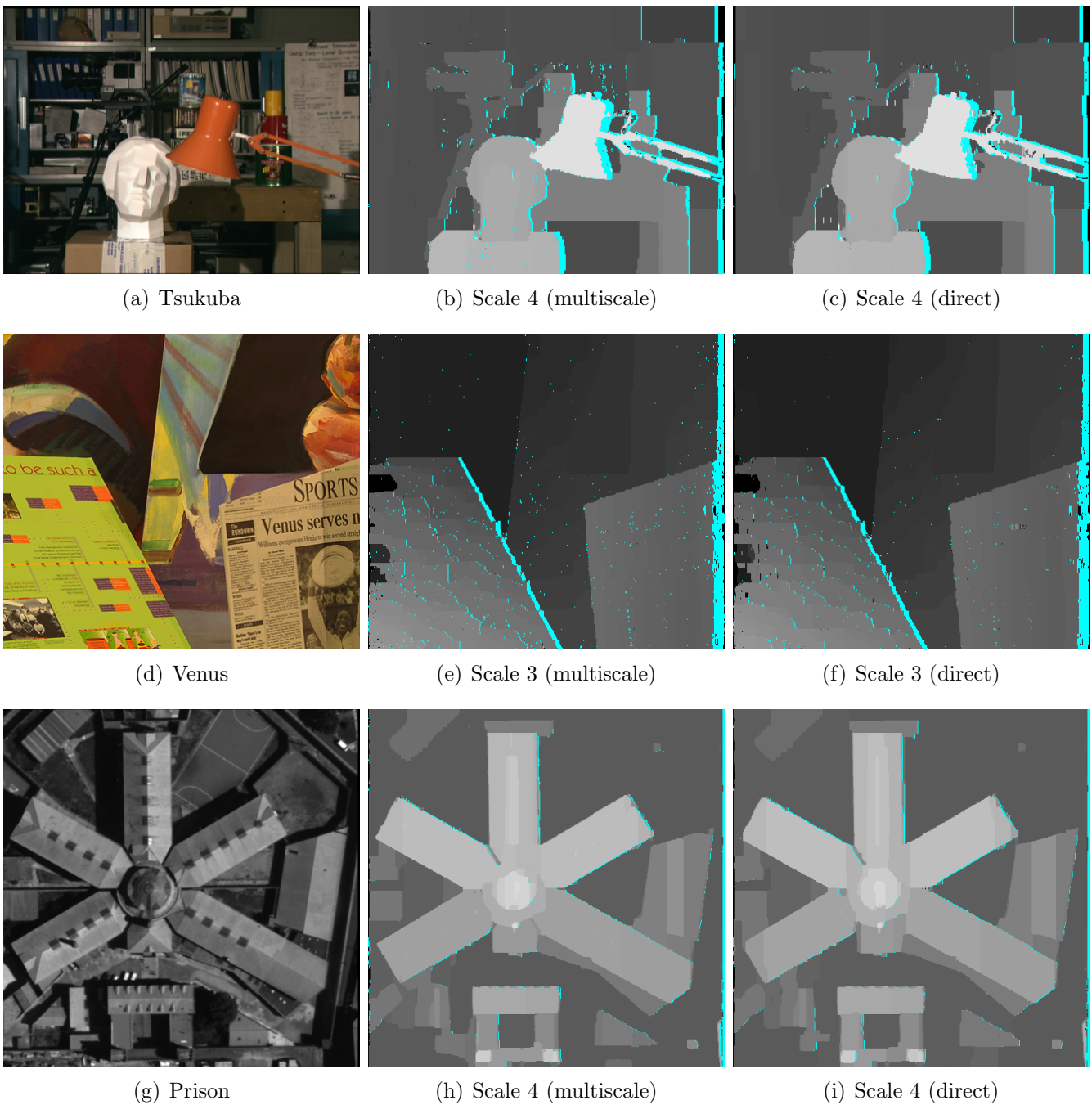
Figure 16: Multiscale approach vs. direct approach in subpixel accurate estimation.
