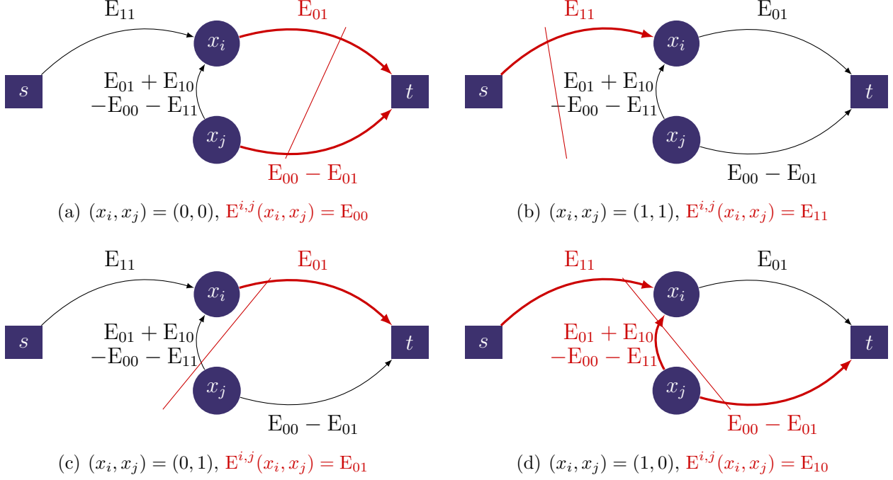
Figure 18: Cuts for the pairwise function as constructed in Section 3.1.2.
