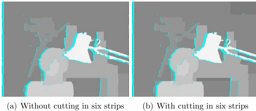
Figure 6: Experimental results on the entire image and the sliced images.
