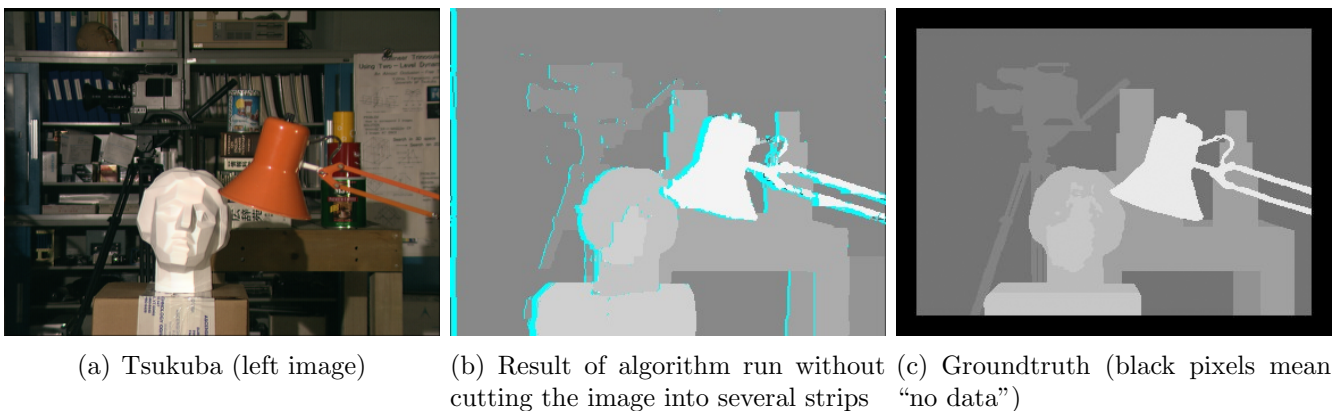
Figure 7: Results of the algorithm on the Tsukuba pair.
