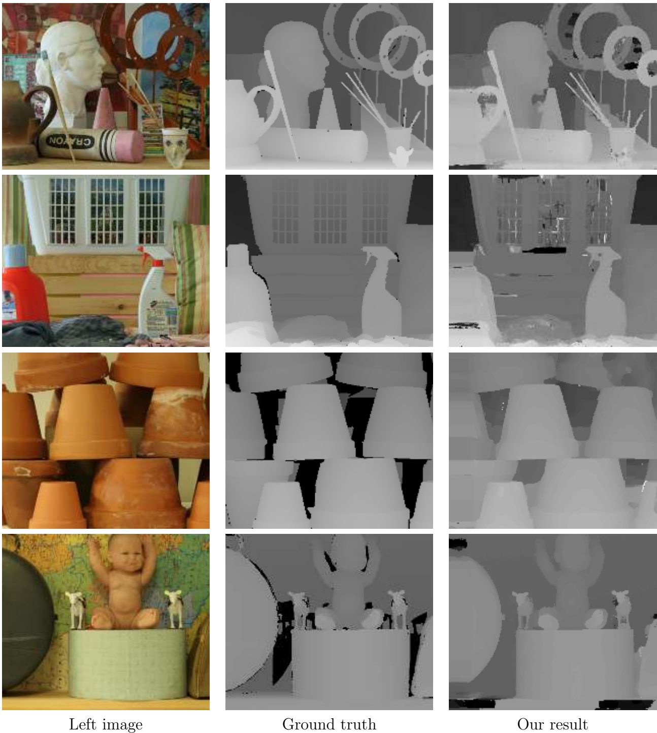
Figure 13: Resulting disparity maps for other images (from top to bottom: Art, Laundry from Middlebury 2005; Flowerpots, Baby3 from Middlebury 2006).
