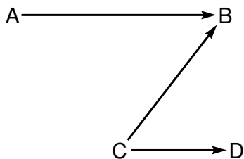
Figure 13: A configuration of edge points which may lead to different chaining results depending on the order of exploration. The potential chains among points A , B , C and D are drawn by arrows. The distances satisfy \|A - B\| > \|B - C\| > \|C - D\| . The resulting chaining when the order of exploration is A then B then C will differ from the result when the order of exploration is C then B then A . See the main text.
