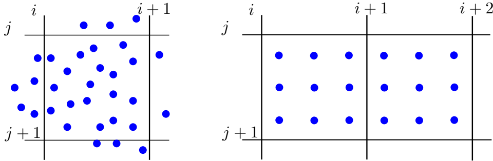
Figure 2: Left: an example of a pixel p such that N = 30 , where the contributions c_n are distributed according to a random process simulated by the renderer. This kind of distribution is used for the creation of the high resolution image. Right: an example of a pixel whose contributions are evenly distributed when N = 9 . This regular distribution is used for the creation of ground truths as disparity maps, occlusion maps and points clouds.
