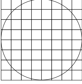
(a) Cartesian sampling of the unit disk
