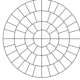
(b) Polar sampling of the unit disk
