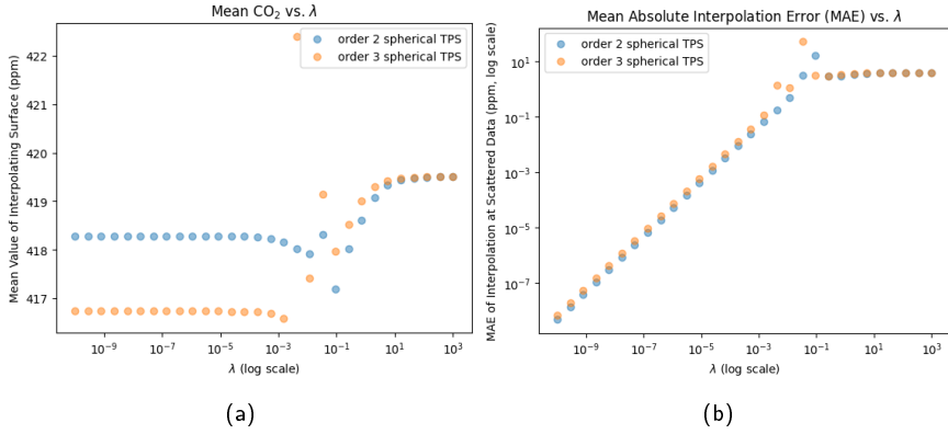
Figure 7: (a) A plot of the global mean CO 2 of the interpolating surface as a function of the regularization parameter \lambda used in constructing it. With low values of \lambda , the order 2 and order 3 spherical splines interpolate the data and, due to their different wiggleness penalties, form different interpolating surfaces with different mean concentrations of CO 2 to do so. With high values of \lambda , the order 2 and order 3 spherical splines agree, as they each yield what is effectively an element of \mathcal{H}_0 = \text{span}\{1\} due to the excessive penalty imposed on wiggleness. With high, but not excessive values \lambda , erroneous averages may be found. (b) The mean absolute error in interpolation at the data points increases with the regularization penalty \lambda , until the interpolation surface is essentially constant.
