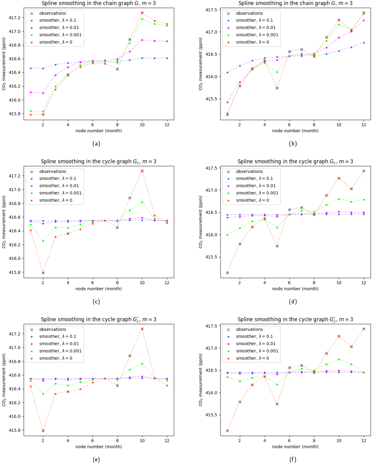
Figure 5: For four distinct choices of wigglyness penalty parameter \lambda , (a) , (c) , and (e) give the smoothing splines after observing nodes \{2, 4, 8, 9, 10\} ; (b) , (d) , and (f) , after observing all nodes 1-12. The top row corresponds to the chain graph G (Figure 2, all edge weights 12); the middle, G_c (Figure 3, edge weights 12); and the bottom, G'_c , which is G_c but with w(t_1, t_{12}) set to 144 to further penalize the non-periodicity of the smoothing splines.
