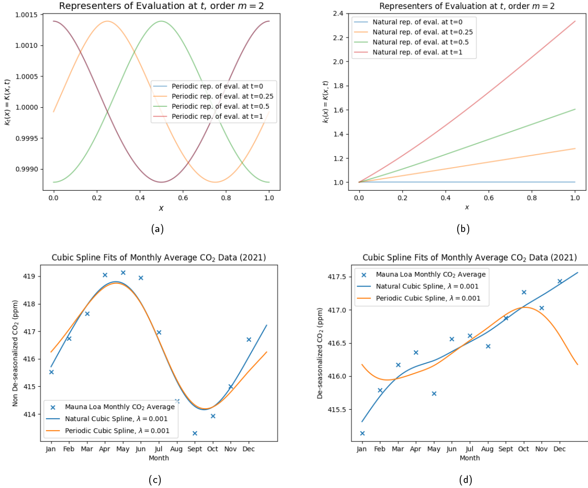
Figure 1: (a) plots the representers of evaluation k_t = k_t^0 + k_t^1 = k(\cdot, t) of the spline on the circle (cubic spline with periodic boundary conditions) at t = 0, 0.25, 0.5 , and 1 . In this case k(\cdot, 0) and k(\cdot, 1) coincide. (b) does the same, but with the kernel for the natural cubic splines. While the kernels are quite different (the former is periodic, treating points with small along-the-circle distance similarly; the latter is cubic up till t , then linear), their Gram matrices' spectra are alike with few, regularly spaced data points. (c)-(d) compare the corresponding spline curves with \lambda = 0.001 on the twelve monthly average CO 2 measurements taken in 2021 at the Mauna Loa station of the Global Monitoring Laboratory network [27], both the untreated data (left), with a naturally occurring periodic component, and the de-seasonalized data (right), reflecting increasing atmospheric CO 2 concentrations. To avoid delving into the complexities of the signal processing chain that produces these monthly averages from discrete measurements, we take these monthly averages to be samples at times t_i = (i - 1) \frac{1}{12} for i \in \{1, \dots, 12\} . Of course, monthly averages are bounded linear functionals, so the representer theorem (Section 2.5) can be applied to more complicated monthly averaging operators L_i than taking a single sample at each t_i .
