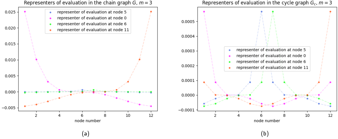
Figure 4: (a) plots the representers of evaluation in \mathcal{H}_1 (with order m=3 ), i.e. k_t^1 = k^1(\cdot, t) , of the kernel k^1 associated with the chain graph G (shown in Figure 2) on \mathcal{X} = \{1, \dots, 12\} at t = 1, 6, 7 , and 12 . (b) gives the same, but for the kernel associated with the cycle graph G_c (shown in Figure 3). In both cases, all edges assume the same weight (12). Dashed lines interpolating between the nodes are included as a visual aid but carry no meaning.
