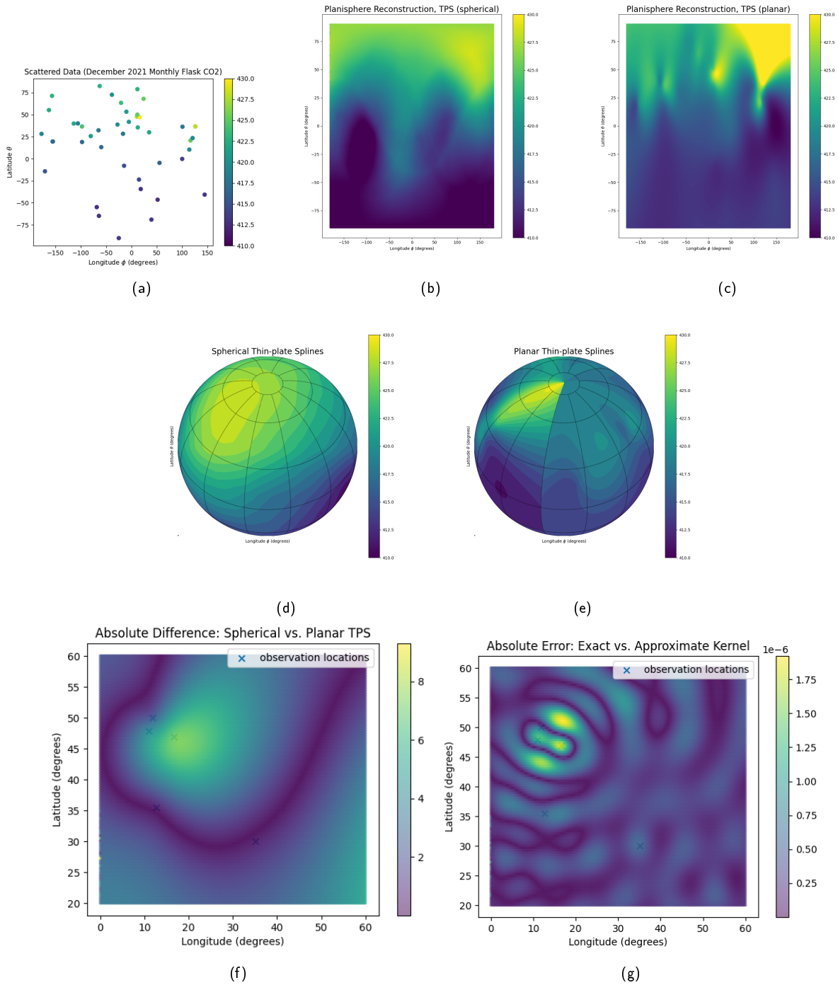
Figure 6: (a) Scattered data of December 2021 monthly averages of flask-air CO 2 readings at 44 sites in the Global Monitoring Laboratory network 50 . (b)-(c) Spherical and planar thin-plate spline fits of these data, respectively, both of order 2. The planar interpolation surface lacks longitudinal periodicity. (d)-(e) display samples of the same surfaces as in (b)-(c) , respectively, but these sample points, uniformly spaced in the plane under an equirectangular projection, are mapped back onto a sphere, which throws into relief the meridional discontinuity of planar thin-plate interpolating surface. In the top-right corner of (c) , the interpolating surface, outside the convex hull of the planar control points, loses its curvature. (f)-(g) show the differences between the spherical and planar thin-plate splines, trained on all 44 points, in their reconstruction of a mesh of points between 0° E and 60° E longitude, and 20° N and 60° N longitude.
