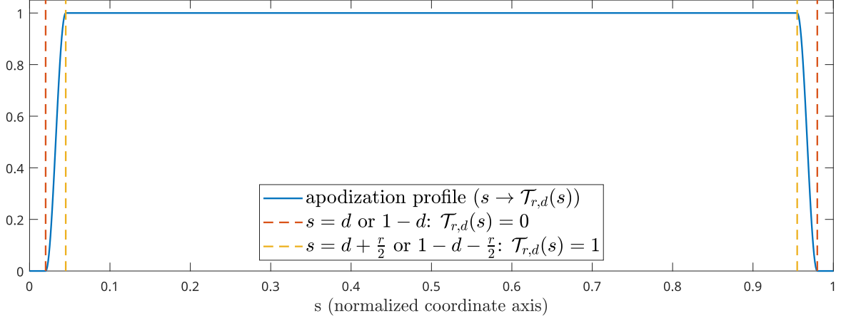
Figure 2: Graph of the one-dimensional apodization profile \mathcal{T}_{r,d} , here represented for r = 5\% and d = 2\% . This function smoothly increases from 0 to 1 over the set [d, d + \frac{r}{2}] , and symmetrically, decreases from 1 to 0 over the set [1 - d - \frac{r}{2}, 1 - d] .
