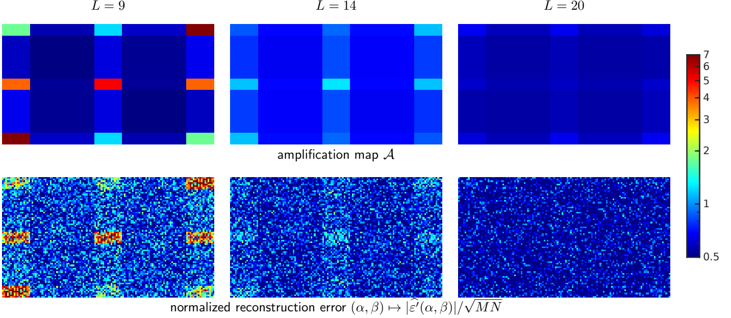
Figure 4: Amplification map and reconstruction error in the Fourier domain. First row: the amplification map \mathcal{A} defined in Proposition 6, for different values of L , \sigma = 1 , random translations uniformly and independently distributed over [-5, 5]^2 , and super-resolution factors equal to z_x = M/m = 129/56 \approx 2.3 and z_y = N/n = 73/33 \approx 2.2 respectively. Second row: the corresponding normalized reconstruction error |\hat{\varepsilon}'|/\sqrt{MN} in the Fourier domain (for one realization of \varepsilon ). We can see that the amplification map gives a good prediction of the fluctuations of |\hat{\varepsilon}'| , and that the amplitude of these fluctuations quickly decreases when L increases. When L is close to z_x z_y (left column), the amplification map may exhibit strong variations from one region to another, which leads to the appearance of some textured error patterns in the reconstructed image (see Figure 5). In most practical cases, however, one has L \gg z_x z_y and the amplification map \mathcal{A} is almost constant (and takes small values).
