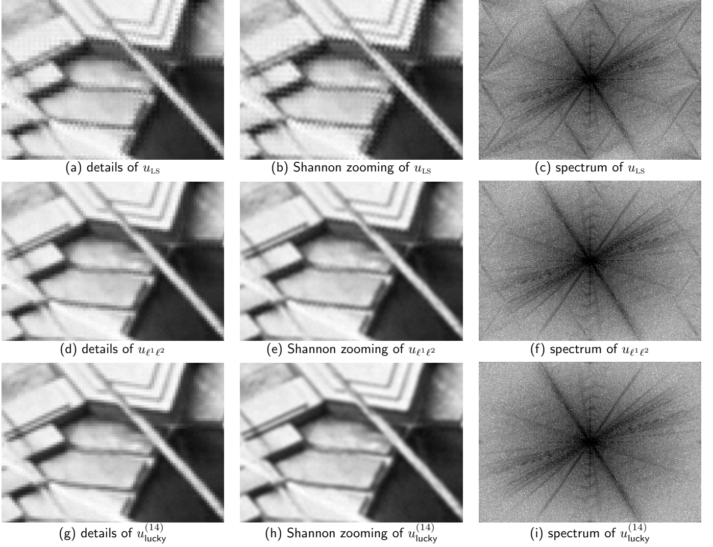
Figure 14: Super-resolution in the presence of outliers. We processed the sequence u_0 ( L = 20 images) using the perturbed displacements \delta' described in Figure 13. Due to the presence of strongly inaccurate displacements in \delta' , the least-squares reconstruction u_{LS} obtained from u_0 and \delta' exhibits severe artifacts at the pixel scale (a), at the sub-pixel scale (b) and in the frequency domain (c). As we can see in the second row, those artifacts are attenuated in the image u_{\ell^1 \ell^2} obtained with the IRLS scheme (56). Unfortunately they remain slightly visible at the pixel scale (d), and significantly visible at the sub-pixel scale (e) and in the frequency domain (f). By keeping only 14 well-chosen images from the low-resolution sequence u_0 with the proposed lucky-imaging procedure, we obtain the image u_{lucky}^{(14)} (third row), which is free of artifacts (g)-(i). This experiment illustrates that, although the minimization (54) is more robust than the least-squares minimization (17), it does not completely get rid of the artifacts caused by the presence of outliers in u_0 . Fortunately, the IRLS procedure provides, through the weights that characterize outlier images, a very efficient way to avoid these artifacts with the proposed lucky-imaging procedure.
