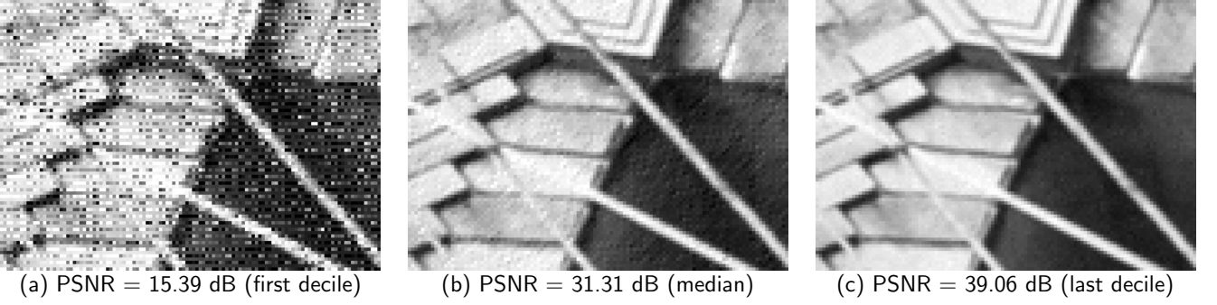
examples of reconstructions using low-resolution stacks containing L = 5 images
