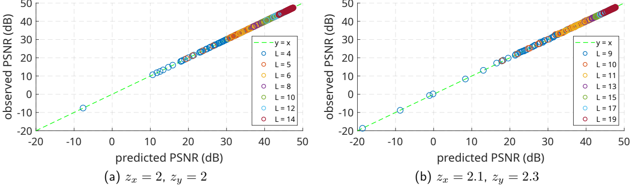
Figure 6: Prediction of the reconstruction PSNR. Here, we illustrate the effectiveness of the error prediction allowed by Corollary 1. For 7 values of L , we simulate several low-resolution sequences (100 per value of L , with random i.i.d. translations uniformly sampled over [-5, 5]^2 , and noise standard deviation \sigma = 2 ) and for each of them we compute the associated super-resolution image with super-resolution factors equal to z_x = M/m = 450/225 = 2 , z_y = N/n = 324/162 = 2 (case a, left column) or z_x = M/m = 450/214 \approx 2.1 , z_y = N/n = 324/141 \approx 2.3 (case b, right column). Then we plot, in each case, a point with x coordinate equal to the PSNR predicted by Equation (46) from the amplification map \mathcal{A} and y coordinate equal to the PSNR measured by comparing the reconstruction u_{LS} to the ideal (apodized) high-resolution image \overline{u_{LS}} . We can observe the high accuracy of the prediction, as all these points are almost perfectly located on the line y = x . Note that the observed PSNR was calculated after removing the small apodization regions on the border of the image domain (otherwise, the apodization would artificially increase the PSNR).
