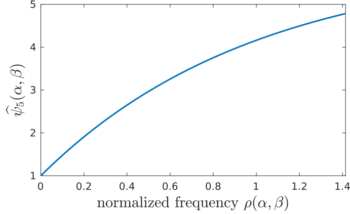
Figure 16: Radial profile (in the Fourier domain) of the enhancement filter \hat{\psi}_5
