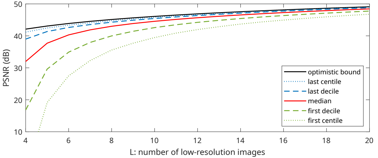
Figure 8: Variability of the reconstruction quality with respect to the number L of low-resolution images. We compute the PSNR of the super-resolved image u_{\text{LS}} obtained from a sequence u_0 of L synthetic low-resolution images (corrupted by an additive Gaussian noise with standard deviation \sigma = 2 and generated using random displacements \delta ). For each value of L , we perform 10^5 simulations and display, as a function of L , the first centile, the first decile, the median, the last decile and the last centile of the computed PSNR values. As the system is (almost surely) overdetermined when L > 4 (that is, the operator A has full rank), we know from Proposition 7 that we can expect to reduce the level of noise by up to a factor \lambda_L = \sqrt{L/(z_x z_y)} = \sqrt{L}/4 , leading to an upper bound for the expected PSNR of 10 \cdot \log_{10} (255^2 / (\sigma / \lambda_L)^2) , which is represented by the black continuous curve (optimistic bound). This PSNR improvement is confirmed by the experiment, especially for large values of L , and it shows the ability of the least-squares to provide substantial denoising in overdetermined situations.
