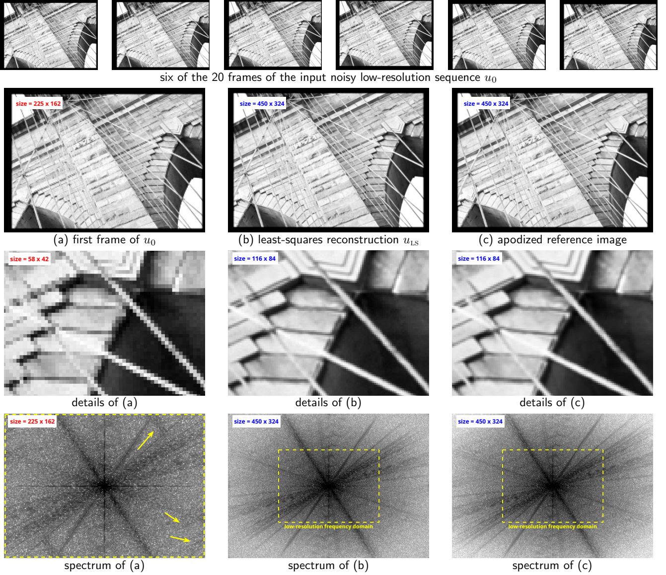
Figure 7: Super-resolution with factor 2 \times 2 using Algorithm 2. In the first row, we display six frames of an apodized synthetic sequence u_0 containing L = 20 noisy low-resolution images. The first frame of u_0 is also displayed in (a). We display in (b) the high-resolution image u_{LS} computed using Algorithm 2, which can be compared to the apodized high-resolution reference image displayed in (c). In the third row, we display some close-up views of the images (a), (b) and (c), and in the last row, we display their Fourier spectra on a logarithmic scale (with high values in dark). The low-resolution image (a) is badly sampled, as attested by the aliasing artifacts appearing in its spectrum (yellow arrows). Comparing (b) and (c), both in the image and the frequency domains, we can see that Algorithm 2 succeeds in reconstructing the high-resolution details of the reference image. Indeed, u_{LS} is very close to the apodized reference image (c), with a relative PSNR equal to 49.0 dB. This experiment illustrates the ability of the least-squares reconstruction model to efficiently recover the high-resolution image from u_0 when L is significantly higher than the targeted total super-resolution factor (here, 4 = 2 \times 2 ), and in the (idealized) case of perfectly known displacements ( \sigma_\delta = 0 ).
