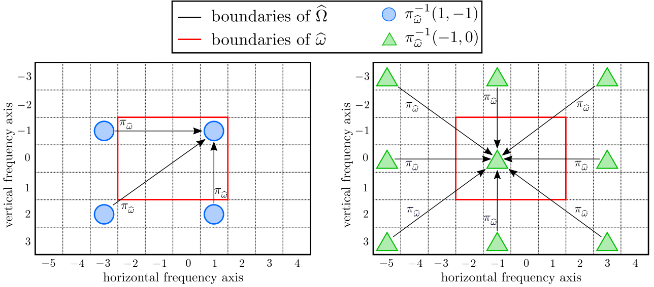
Figure 3: Frequency aliasing with fractional aliasing factors. Here, using a very small image ( M \times N = 10 \times 7 ) we illustrate the effect of subsampling in the Fourier domain. Left: the large black rectangle ( M \times N ) delineates \hat{\Omega} , the Fourier domain of a high-resolution image, u_{\text{HR}} , while the small ( m \times n = 4 \times 3 ) red rectangle delineates \hat{\omega} , the Fourier domain of the low-resolution image u_{\text{LR}} = S_z u_{\text{HR}} (here we have z = (z_x, z_y) = (\frac{10}{4}, \frac{7}{3}) ). Blue points represent all frequencies of the high-resolution image that \pi_{\hat{\omega}} maps onto the low-frequency (a, b) = (1, -1) . In other words, the effect of subsampling a high-resolution image u_{\text{HR}} into a low-resolution image u_{\text{LR}} would result, in the Fourier domain, in
