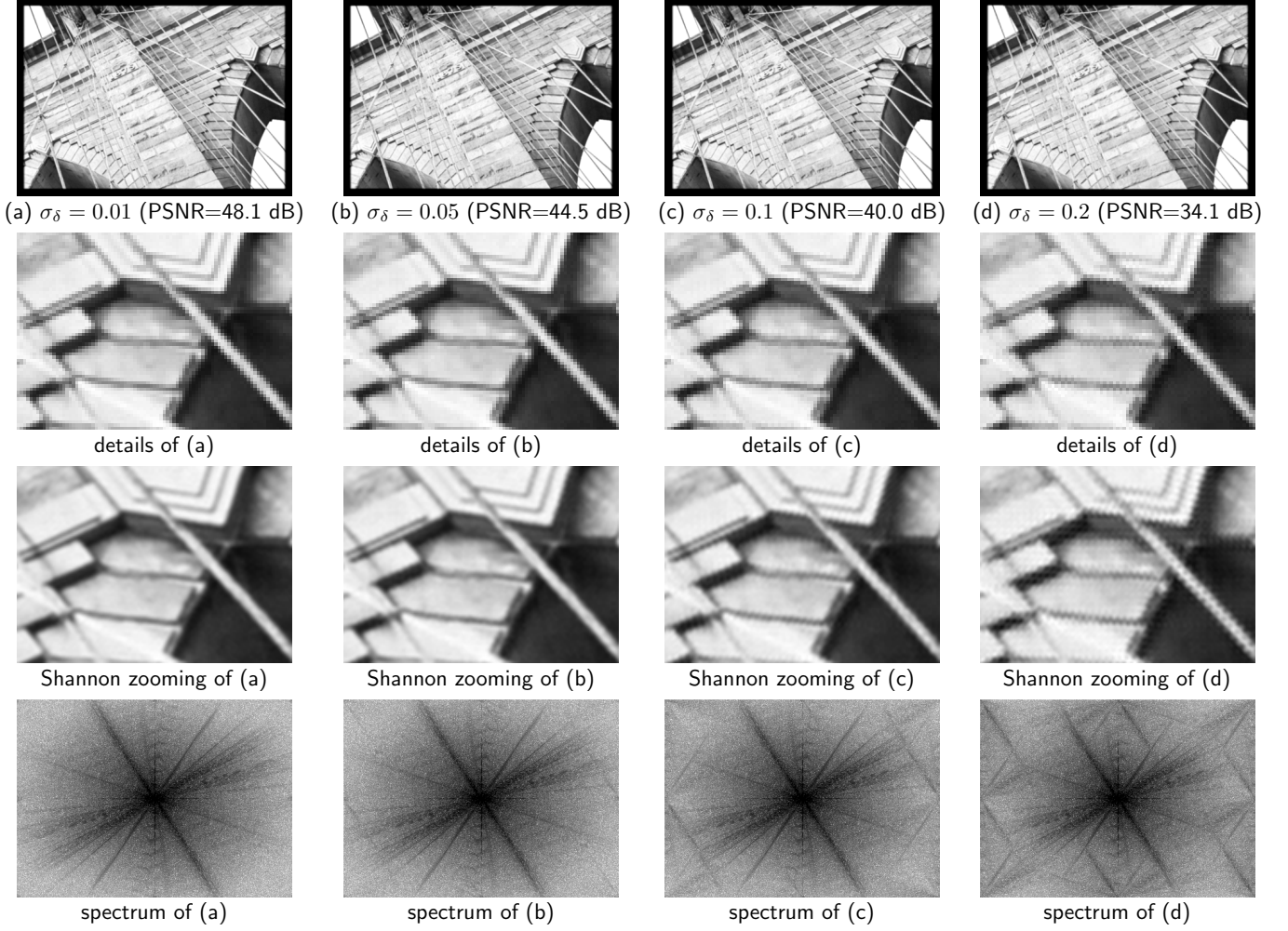
Figure 10: Least-squares reconstruction using erroneous displacements. For each value of \sigma_\delta considered in this figure, we simulated 10^3 synthetic low-resolution sequences in the following way: each sequence u_0 contains L = 20 low-resolution images (corrupted by an additive Gaussian noise with standard deviation \sigma = 2 ) and was generated using a random displacement sequence \delta (drawn with independent and uniform samples in [-5, 5] \times [-5, 5] ). For each simulated sequence, we computed the least-squares reconstruction u_{LS} obtained from u_0 and a perturbed displacement sequence \delta' = (\delta^{(j)} + (n_x^{(j)}, n_y^{(j)}))_{1 \leq j \leq L} with i.i.d. \mathcal{N}(0, \sigma_\delta^2) perturbations (n_x^{(j)}, n_y^{(j)}) ( 1 \leq j \leq L ). In the first row, we display, for several values of \sigma_\delta , the reconstruction u_{LS} achieving the median PSNR with respect to the reference high-resolution image. A close-up is displayed in the second and third rows (with Shannon interpolation in the third row). The last row represents the spectra (on a logarithmic scale) of the high-resolution images (a)-(d). Looking closely at the images at the pixel scale (second row), we can observe some spurious structures in the reconstruction (c) and (d). Looking at the sub-pixel scale (third row), artifacts are clearly visible in (c) and (d), and slightly visible in (b). In the spectra of the reconstructed images (last row), artifacts are clearly visible in (b), (c), (d), but barely in (a). This experiment shows that, for a 2 \times 2 super-resolution factor and a sequence of L = 20 low-resolution images, artifacts are barely noticeable in the image domain when \sigma_\delta \leq 0.05 , but \sigma_\delta \leq 0.01 is required to draw the same conclusion in the Fourier domain.
