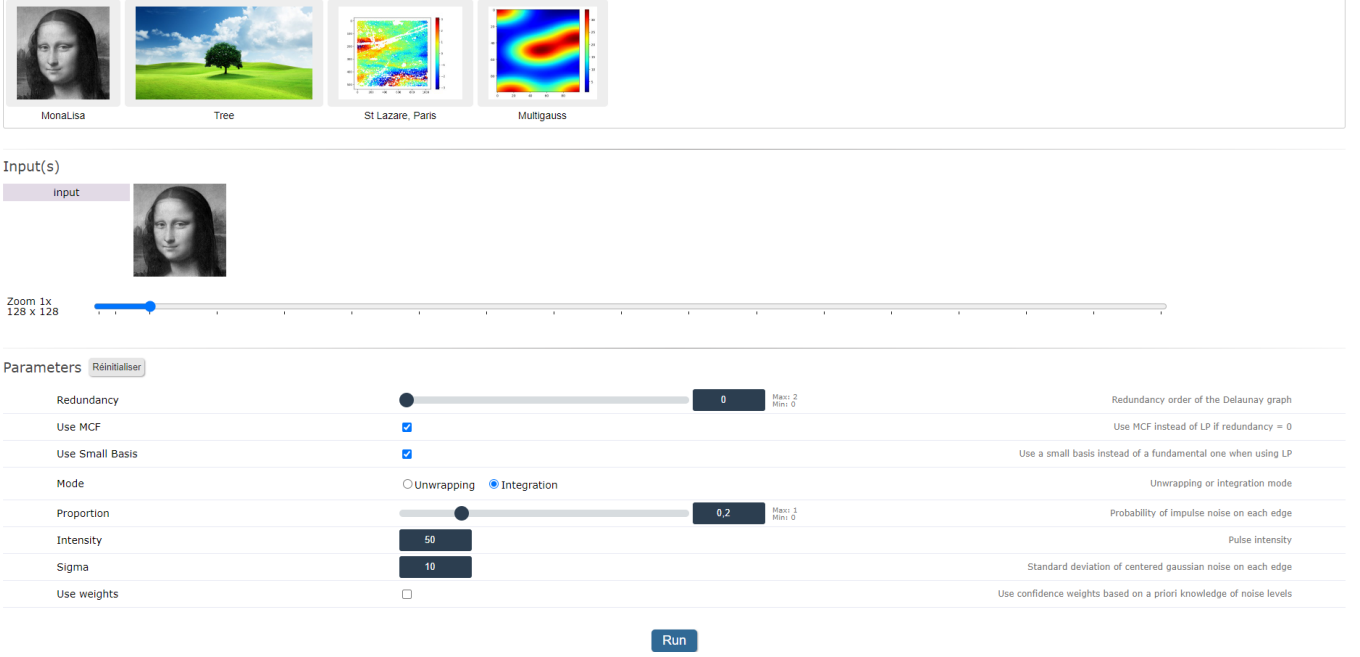
Figure 41: Demo interface in Integration mode
