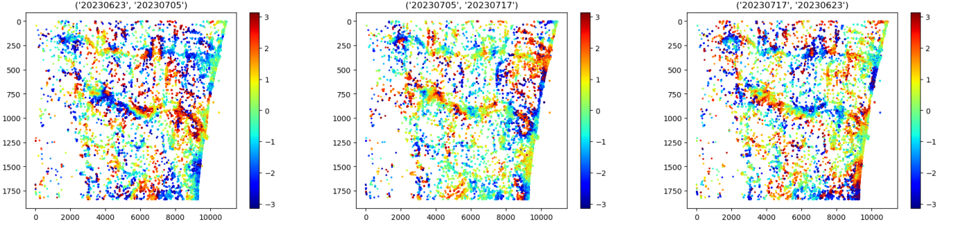
Figure 31: From left to right: wrapped interferograms between dates 2023-06-23/2023-07-05, 2023-07-05/2023-07-17 and 2023-07-17/2023-06-23.
