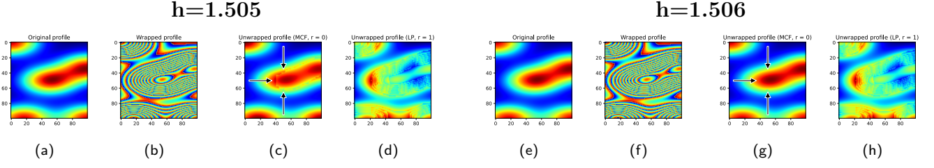
Figure 14: The four leftmost figures (a, b, c, d): h = 1.505 , just before a transition; the four rightmost figures (e, f, g, h): h = 1.506 , past a transition, when r = 0 . Note how a whole region around the two peaks in the middle of the image was corrected using MCF (Figure (c) vs. Figure (g)). Meanwhile, the unwrapped signal when r = 1 is still far from the ground truth (Figure (d) vs. Figure (h)). Note that this is called a transition because normally, while a smaller h makes the unwrapping process easier, such a small difference usually does not change anything (i.e. the error is a continuous function of h almost everywhere). These snapshots show a sizeable difference because it is in an isolated neighborhood of a special, pivotal value of h showing up as the first jump or step in the error plot versus h in the previous Figure 13. For reference, there are 29969 edges at r = 0 and 94580 at r = 1 , which means about \frac{1}{3} of the edges are nonredundant and \frac{2}{3} of the edges are redundant. In both cases ( h = 1.505 and h = 1.506 ), the percentage of wrongly estimated gradients is 4.5% at r = 0 and 20.9% at r = 1 (actually the ratios are slightly different but not up to 10^{-3} ). They are the same in the two blocks because the change in h is so slight that the percentages have not been affected up to a precision of 10^{-3} , yet this change was sufficient to entail a clearly noticeable correction when r = 0 .
