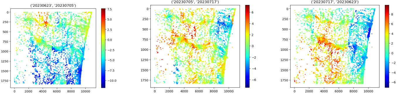
Figure 32: From left to right: unwrapped interferograms between dates 2023-06-23/2023-07-05, 2023-07-05/2023-07-17 and 2023-07-17/2023-06-23, with redundancy 2.
