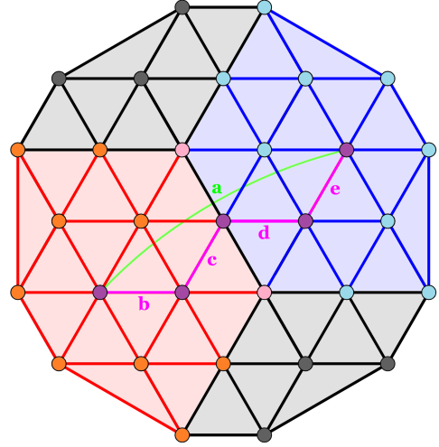
(b) Simple illustration of the creation of a cycle involving a redundant arc a with redundancy 3 in green in a larger Delaunay triangulation. The two breadth-first clusters, in red and blue, intersect after 4 iterations (two for each cluster) and an instance of a possible path completing the cycle is shown in pink. The new cycle corresponding to a is thus cycle (a, b, c, d, e) .
