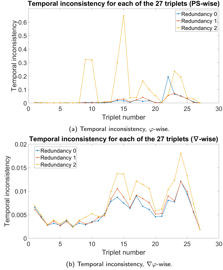
Figure 34: Temporal inconsistency for each of the 27 triplets, numbered chronologically, for each level of redundancy, PS-wise (top) and gradient-wise (bottom).
