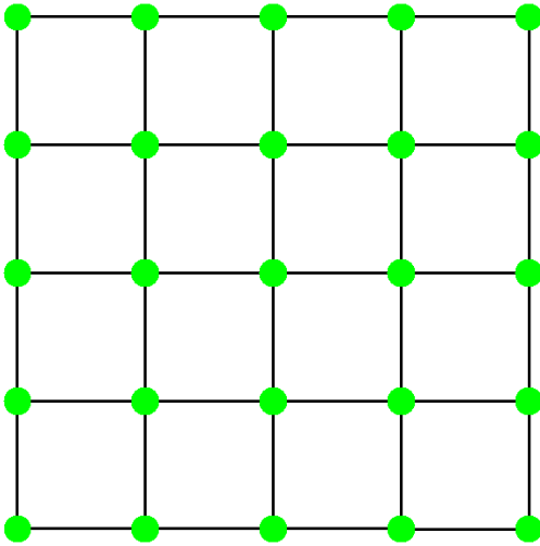
(a) Graph of a regular 5 \times 5 grid.
