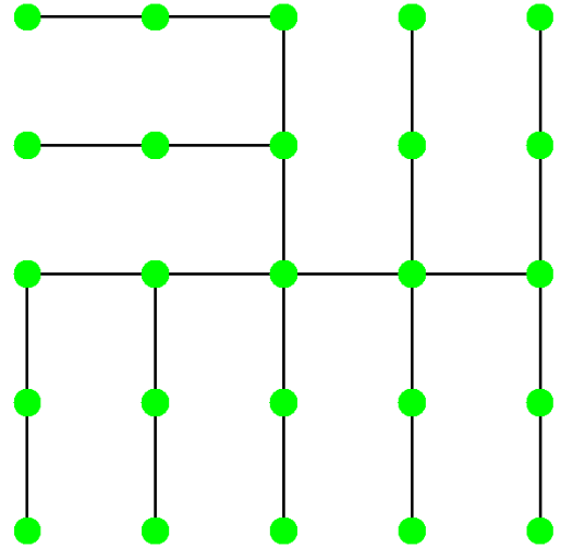
(b) Example of a spanning tree of graph (a)
