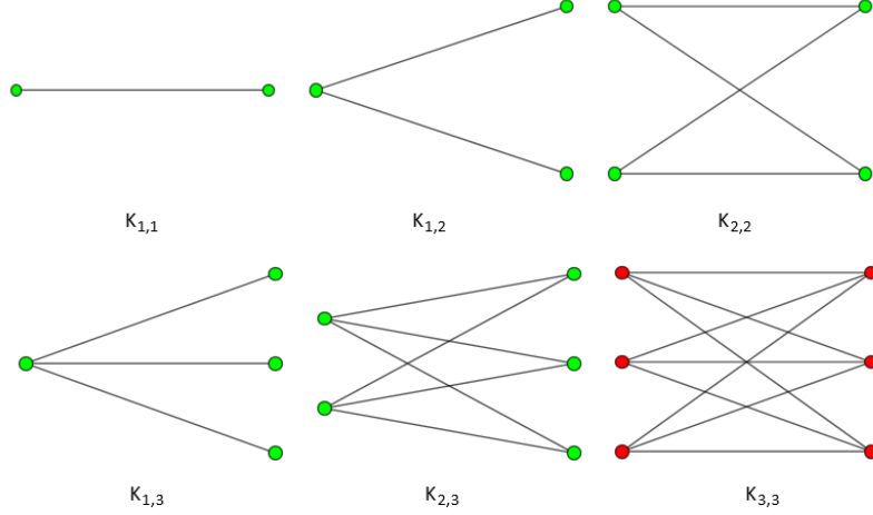
Figure 5: A list of complete bipartite graphs K_{n_1,n_2} for 1 \leq n_i \leq 3 and n_1 \leq n_2 . Planar graphs are drawn with green vertices while non-planar ones are drawn with red vertices. The graphs are drawn using a canonical form, so some graphs can exhibit crossing edges despite their being planar.
