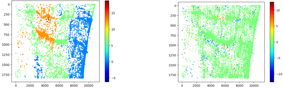
Figure 33: Left: Temporal inconsistency in the interferogram triplet with the worst result PS-wise (50%). This means the error rate is at least \frac{1}{2} . Note that temporal inconsistency is necessarily an integer multiple of 2\pi , and that while (PS-wise) temporal inconsistency is supposed to be zero, this is up to an unknown constant, so it is not possible to be sure where the errors lie. Having more than a single color simply shows there must be errors, with correctly unwrapped points belonging to a single color. Right: corresponding gradient-wise temporal inconsistency (where each point corresponds to an edge of the spanning tree and was placed in the middle of it). Since they are not up to a constant, a properly unwrapped (error-free) gradient must show up as zero on the graph, otherwise, an unwrapping mistake has been made. Note that a few gradient-wise errors can induce PS-wise errors in a large region.
