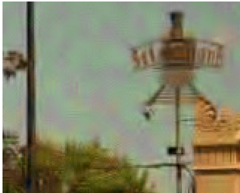
DCT denoising
