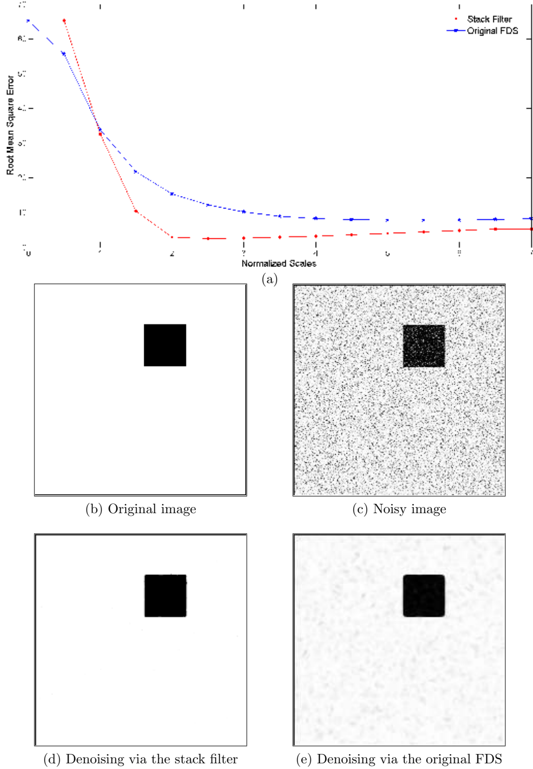
Figure 18: Denoising properties of the stack filter and of the original FDS when p = 20\% .
