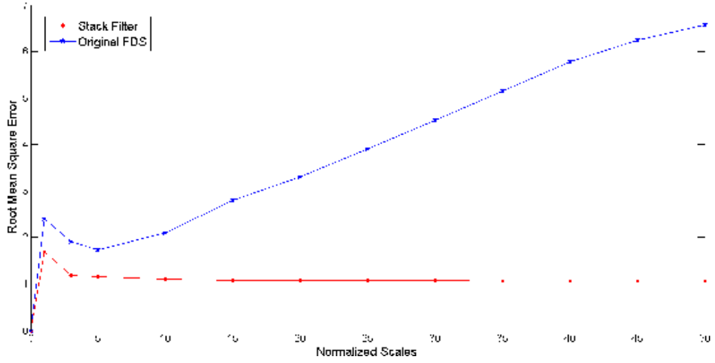
Figure 7: Contrast invariance test for the stack filter and the original FDS when g is a quadratic function.
