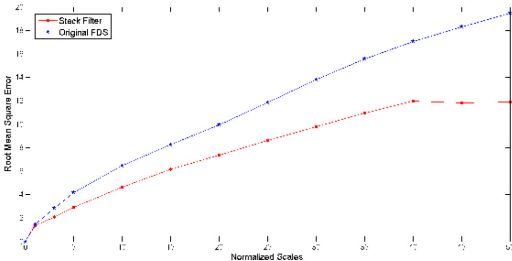
Figure 9: Contrast invariance test for the stack filter and the original FDS if we apply a uniform equalization.
