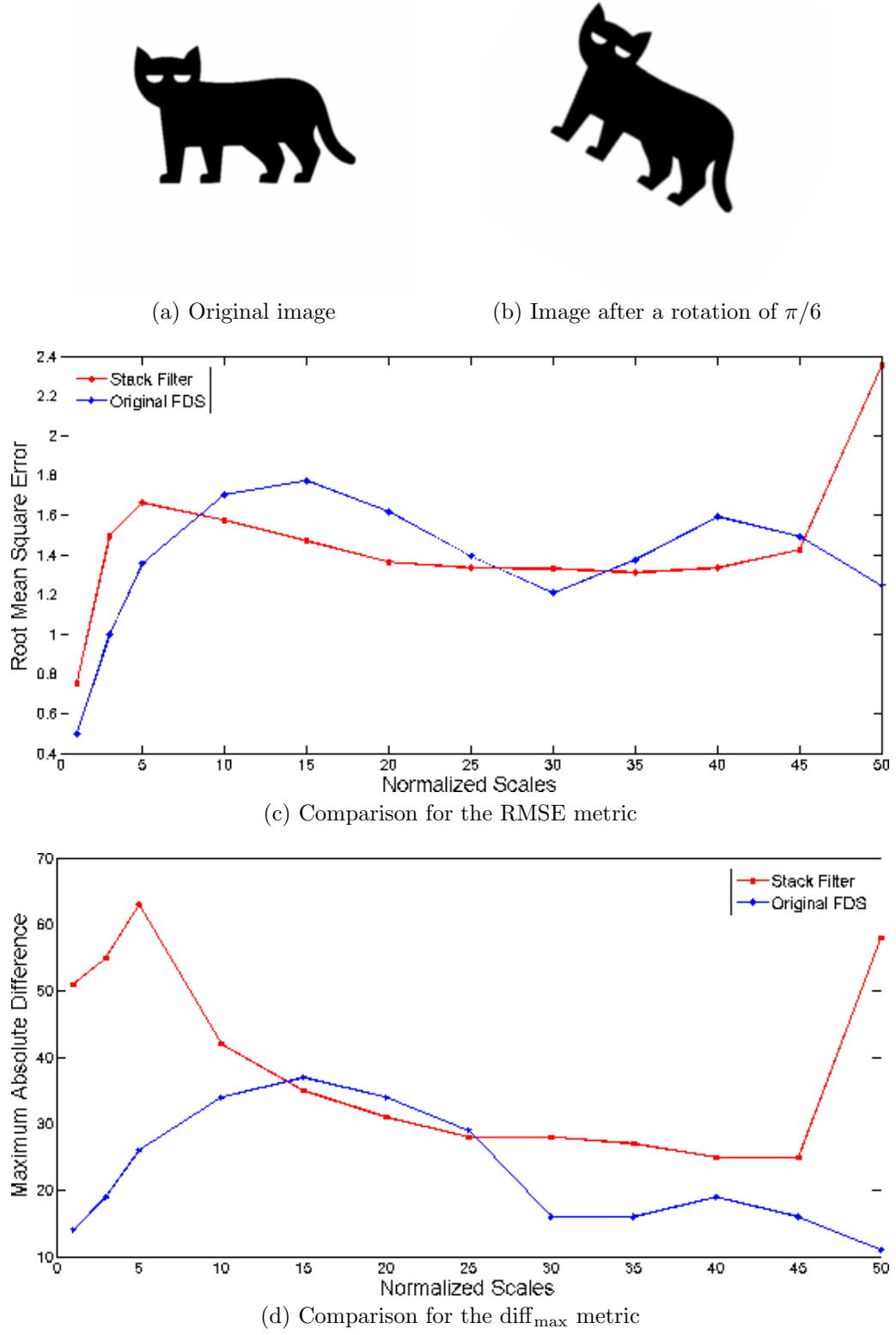
Figure 10: Euclidean invariance test for the stack filter and the original FDS when the transformation f is a rotation of \pi/6 and the input image is almost binary.
