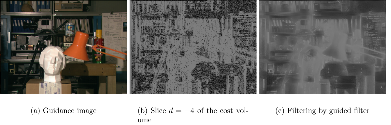
Figure 4: Filtering by guided filter of a slice of the cost volume for the Tsukuba pair ( \tau_1 = 7 , \tau_2 = 2 , \alpha = 0.9 , \varepsilon = 10^{-4} , r_{\text{GF}} = 9 ).
