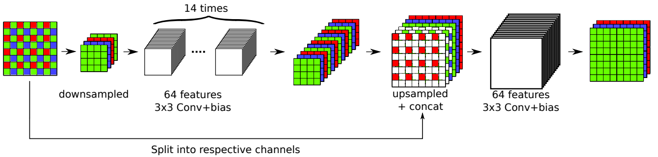
Figure 1: Architecture used for demosaicking by Gharbi et al. [3].
